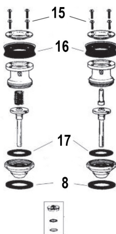
Old Style Brass Piston Assembly Closet Urinal
