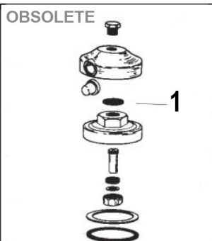
Old Style Brass Piston Assembly Closet Urinal
